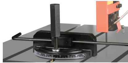
Miter Gauge for Hydraulic Table Shown
