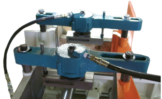
BUNDLE CLAMPS
